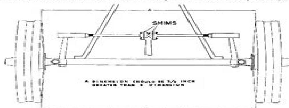
Fig. MH108—Front wheel tie-in—on standard models.
