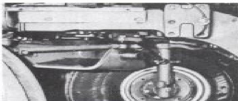
Fig. 351—To remove the main hydraulic pump, disconnect one tie rod and pivot axle support out of way as shown.
