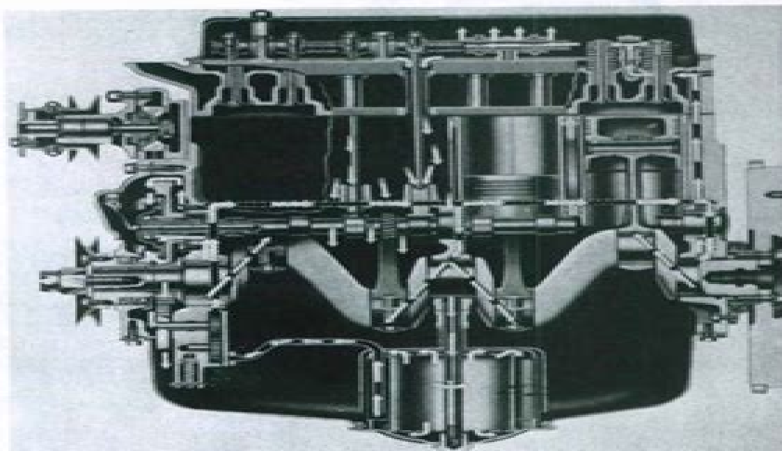
Fig. F4—Models TE20 and TO20 engines.
