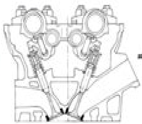
Cylinder head section
