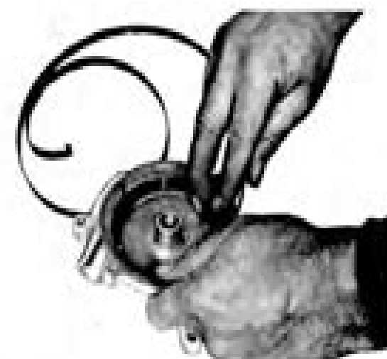
Figure VII-12. Wind the starter spring into the base in a counterclockwise direction. Spring ends are purposely annealed to assist in making spring conform to drum and base at the anchor ends.
