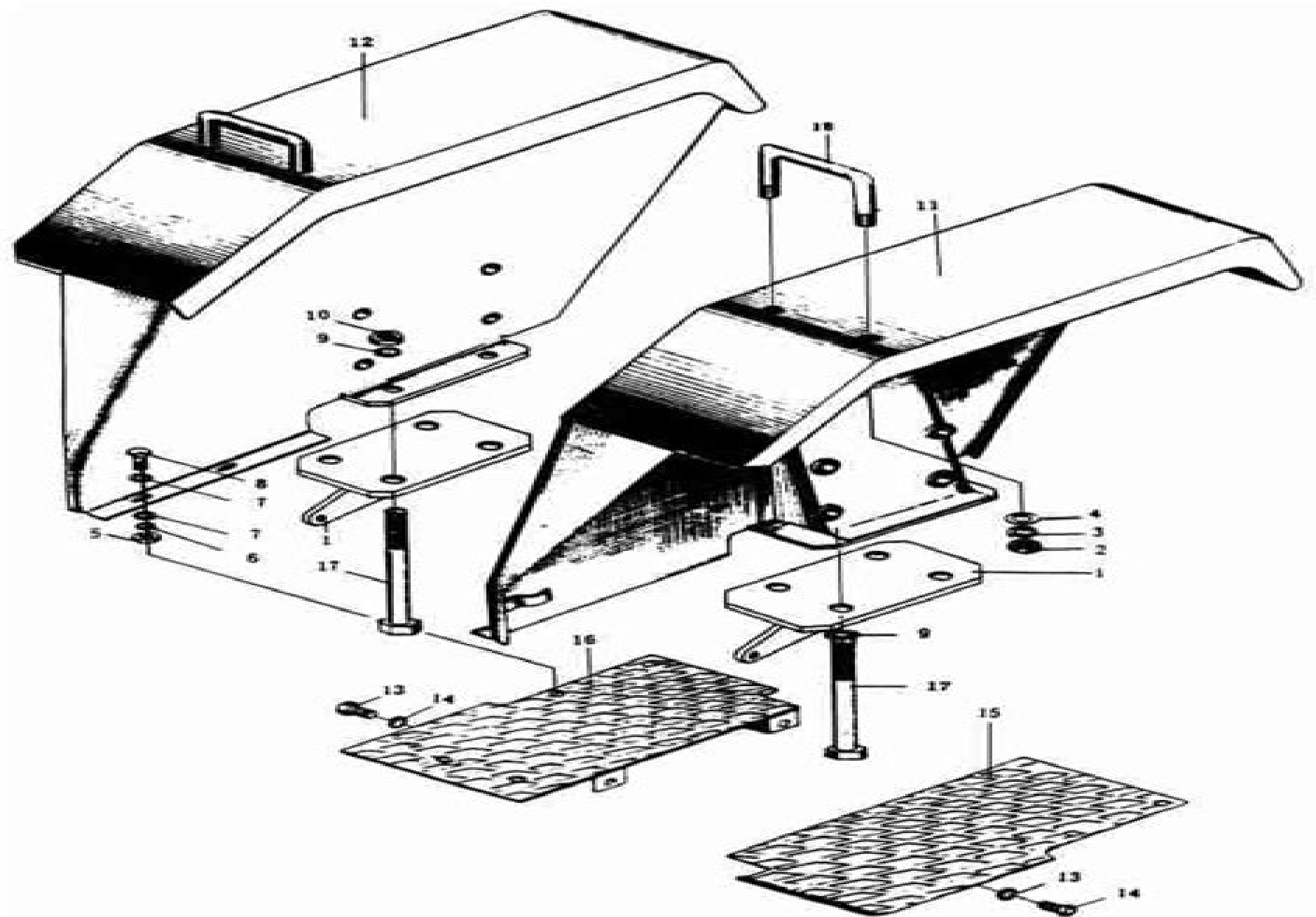
Fig. 15 Mud Shield And Step
