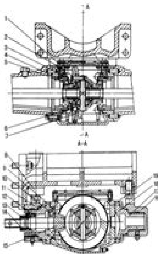
Fig.4-9 Main drive of front drive axle and differential assy
