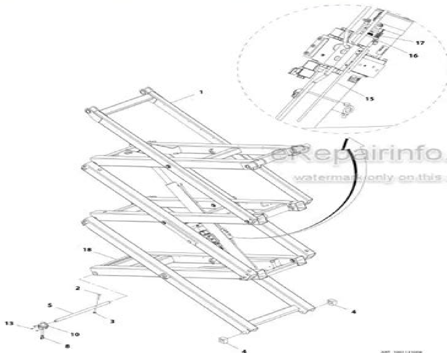
FIGURE 3-1. SCISSORS ARMS INSTALLATION - 1930ES STANDARD HYDRAULIC OIL
