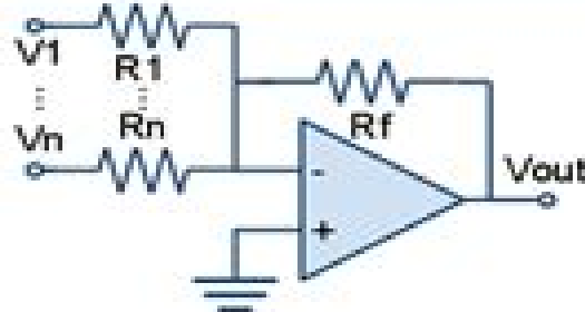
Inverting Summing Amplifier
