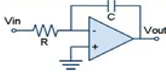
Integrator Amplifier
