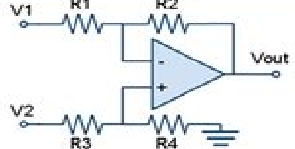
Differential Amplifier
