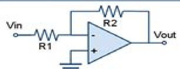
Inverting Amplifier
