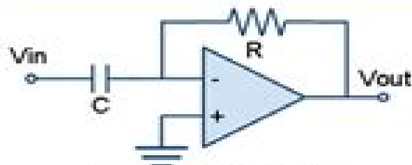
Differentiator Amplifier
