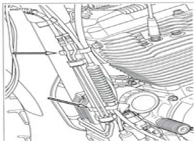
Figure 1-17. Cable Retaining Clips
