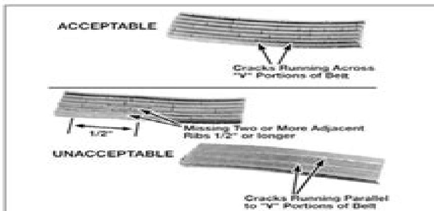
12.4 Small cracks in the underside of a V-ribbed belt are acceptable - lengthwise cracks, or missing pieces that cause the belt to make noise, are cause for replacement
