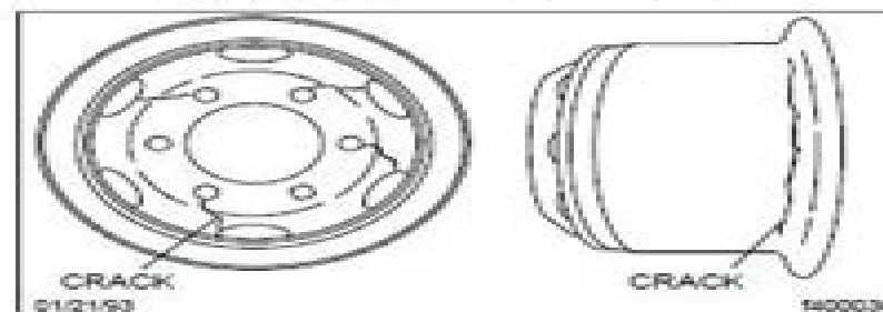
Fig. 2, Cracked Wheel and Rim
