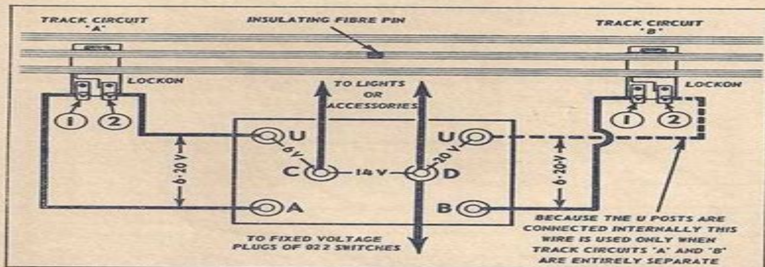
Figure 3—Transformer Connections for Layouts with Two Trains.
