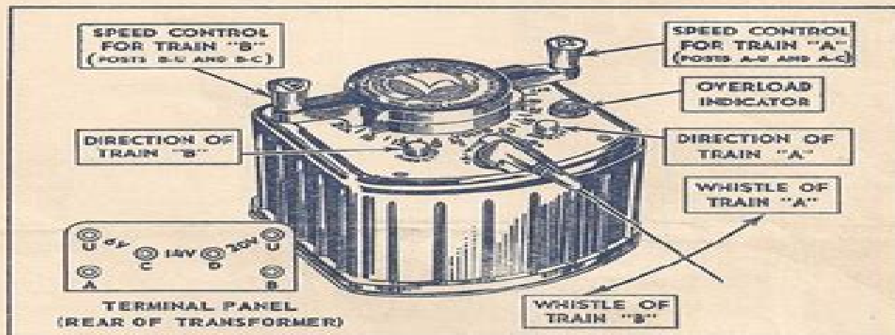
Figure 1—Type "KW" Multi-Control Transformer
