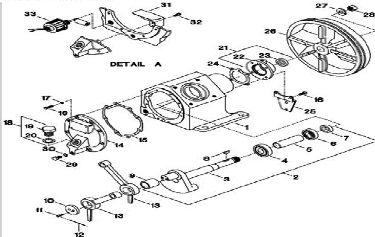
FIGURE 1. COMPRESSOR FRAME ASSEMBLY.
