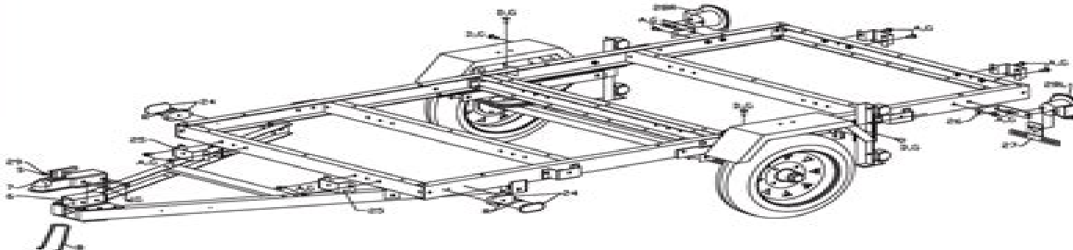
Figure I: Coupler and Stake Clamp Attachment
