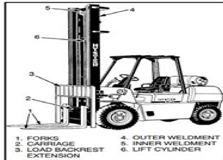
FIGURE 1. MAST COMPONENTS.
