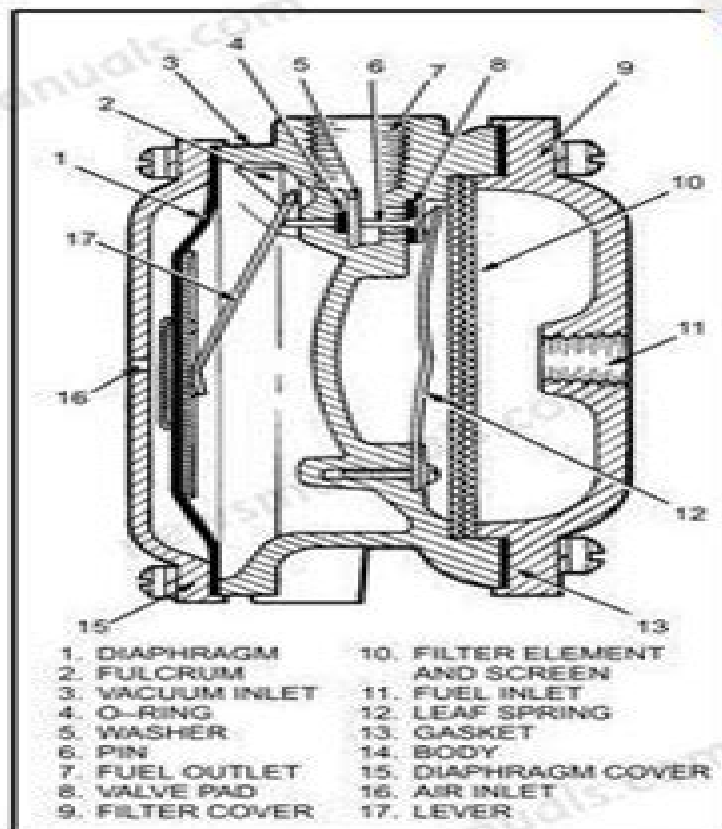
FIGURE 3. FUEL FILTER AND FUEL VALVE
