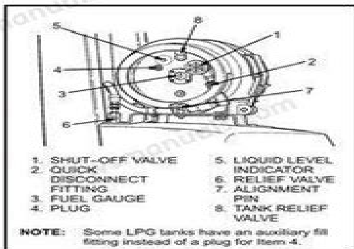
FIGURE 2. LPG TANK
