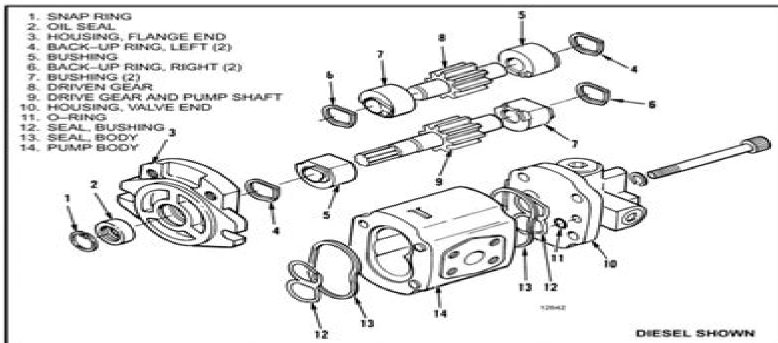
FIGURE 3. HYDRAULIC PUMP ASSEMBLY
