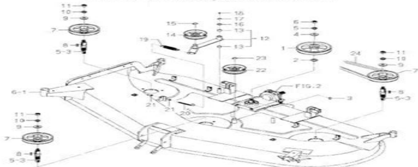
FIG. 3 PULLEY,BELT SYSTEM
