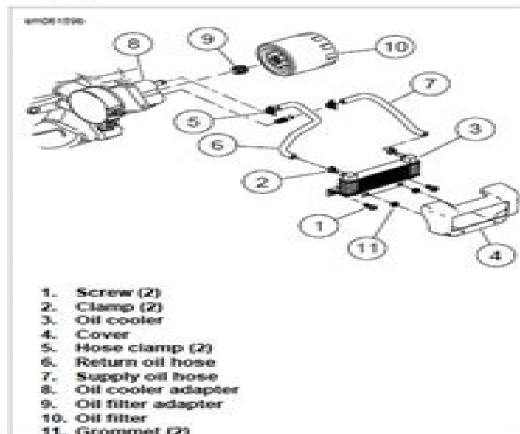
Figure 3-11. Oil Cooler
