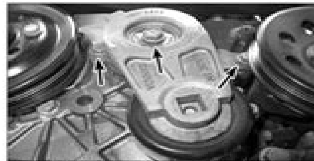
24.25 Typical V6 tensioner mounting fastener locations
