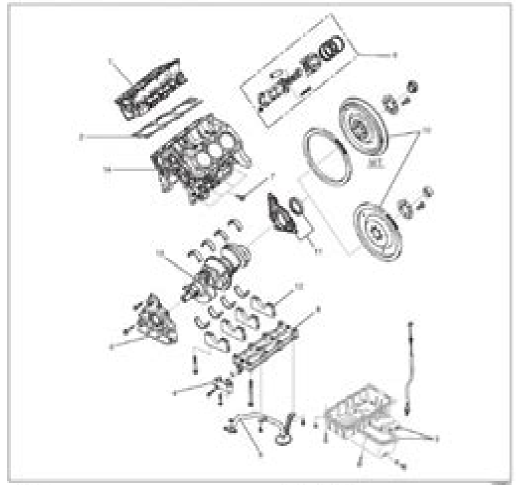
Cylinder Block and Associated Parts
