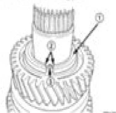
Fig. 18 TWO-PIECE THRUST WASHER
