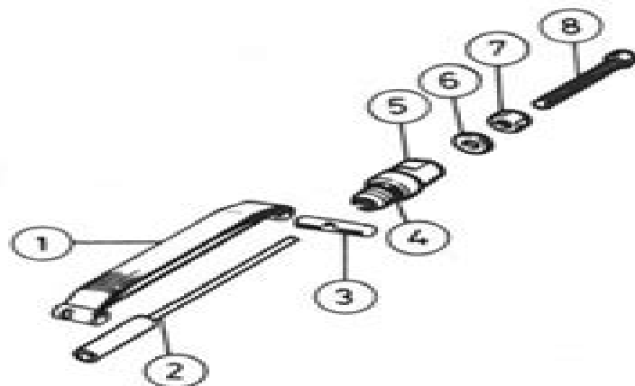
Fig. 9.3 Post 1980 primary chain tensioner assembly
