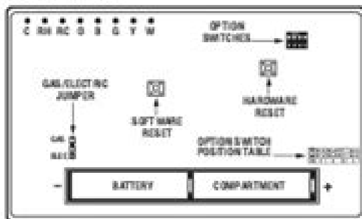
REAR OF THERMOSTAT WITH COVER REMOVED
