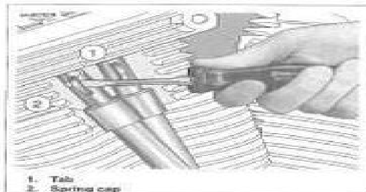
Figure 3-15. Removing Spring Cap Retainer
