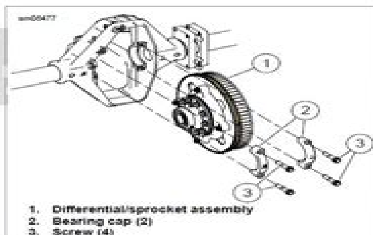
Figure 5-9. Differential and Sprocket Assembly
