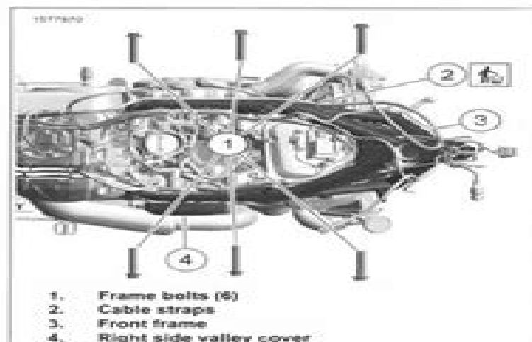
Figure 3-151. Front Frame
