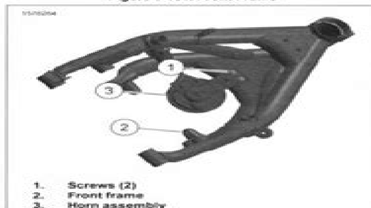
Figure 3-152. Remove Horn Assembly
