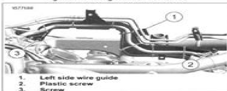
Figure 3-150. Left Side Wire Guide
