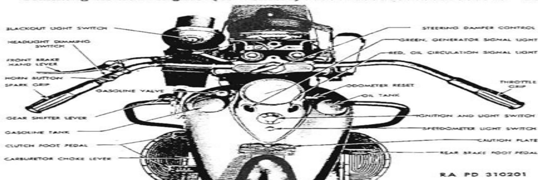
Figure 4—Controls
