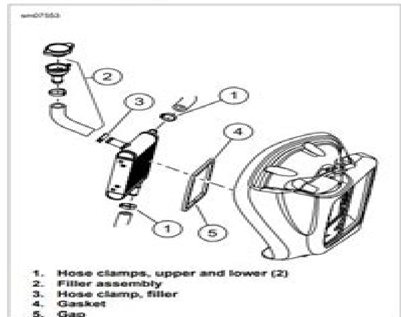
Figure B-10. Radiator
