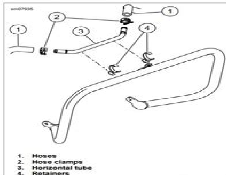
Figure B-9. Coolant Horizontal Line
