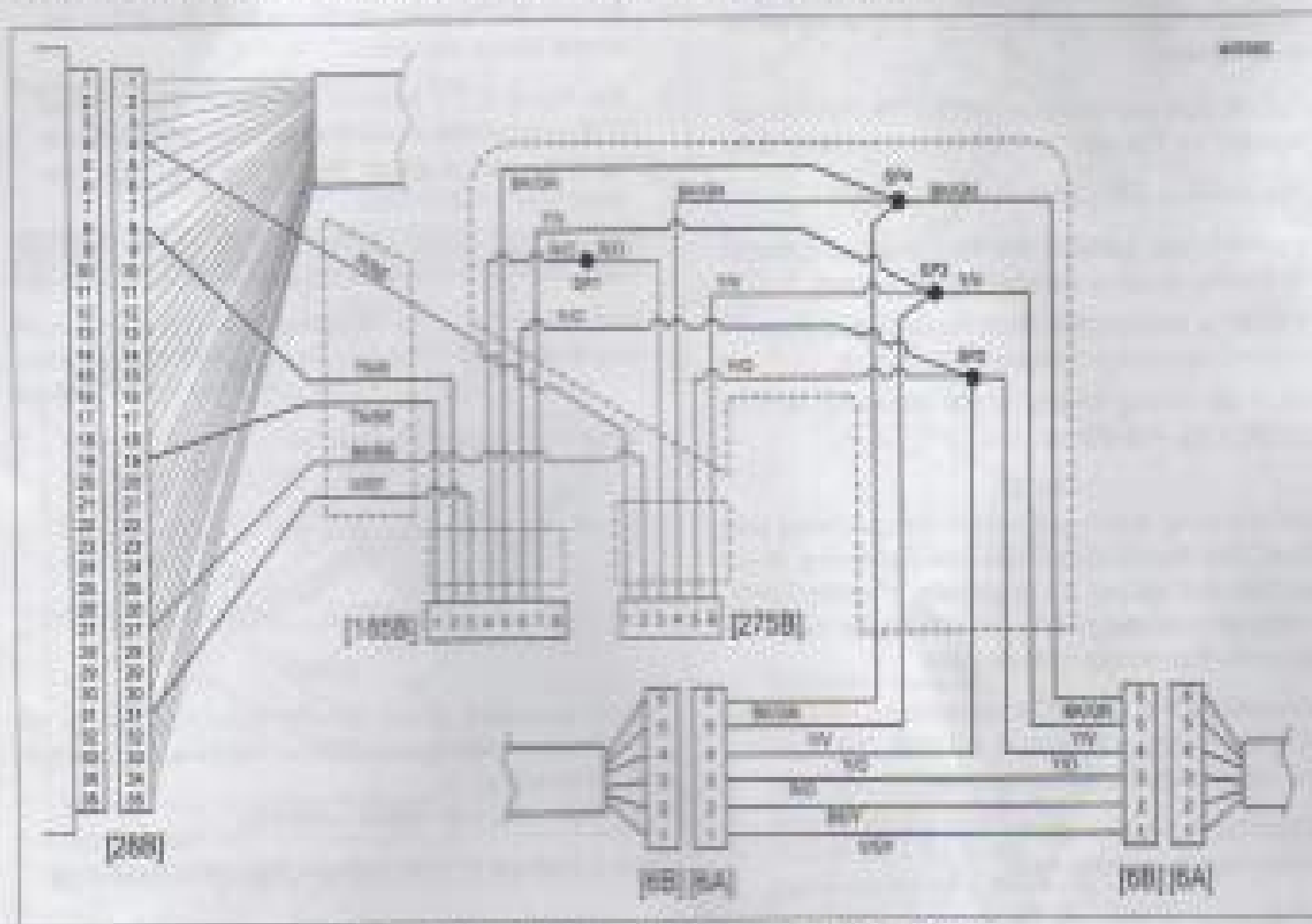
Figure 4. Wiring Diagram, PostNavigation Interface Module
