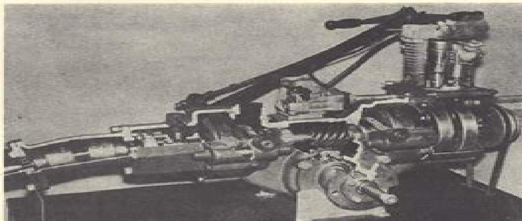
Fig. GR2—Cutaway of Gravelly power plant showing Tee head engine having double internal flywheels, detachable main journals and crankpin and two-piece crankcase.
