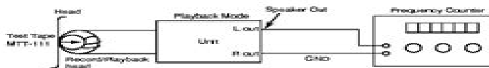
Figure 2. Motor Speed Adjustment Connection Diagram
