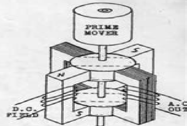
Note solid core in D.C. field coils.
