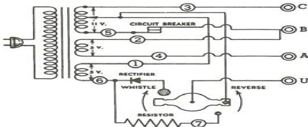
SCHEMATIC WIRING DIAGRAM OF TRANSFORMERS N 22 , 1032, 1033, 1032M and 1232
