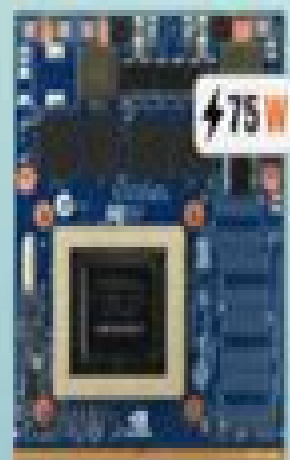
GTX 965M MXM 3.0s GPU 82x105mm
