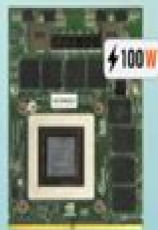
Quadro K3100M MXM 3.0s GPU 82x105mm
