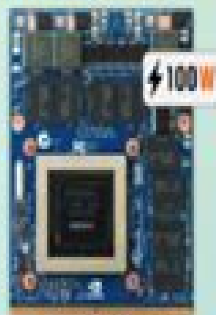
GTX 980M MXM 3.0s GPU 82x105mm
