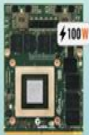
Quadro K5100M MXM 3.0s GPU 82x105mm
