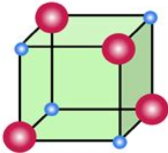
Unit Cell
