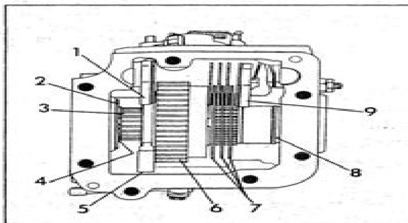
FIG. B.X/22 TOP VIEW, REDUCTION GEARBOX 1. Front plate; 2. Deflector; 3. Sliding sleeve; 4. Snap ring; 5. Shifting pad; 6. Gear; 7. Friction disc; 8. Bevel ring
