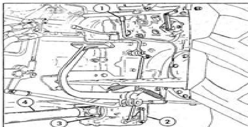
FIG. B.X/20 REDUCTION GEARBOX INSTALLED 1. Control lever, shift forward to engage, rearward, disengage; 2. Reduction gearbox; 3. Cardan shaft screws; 4. Cardan shaft
