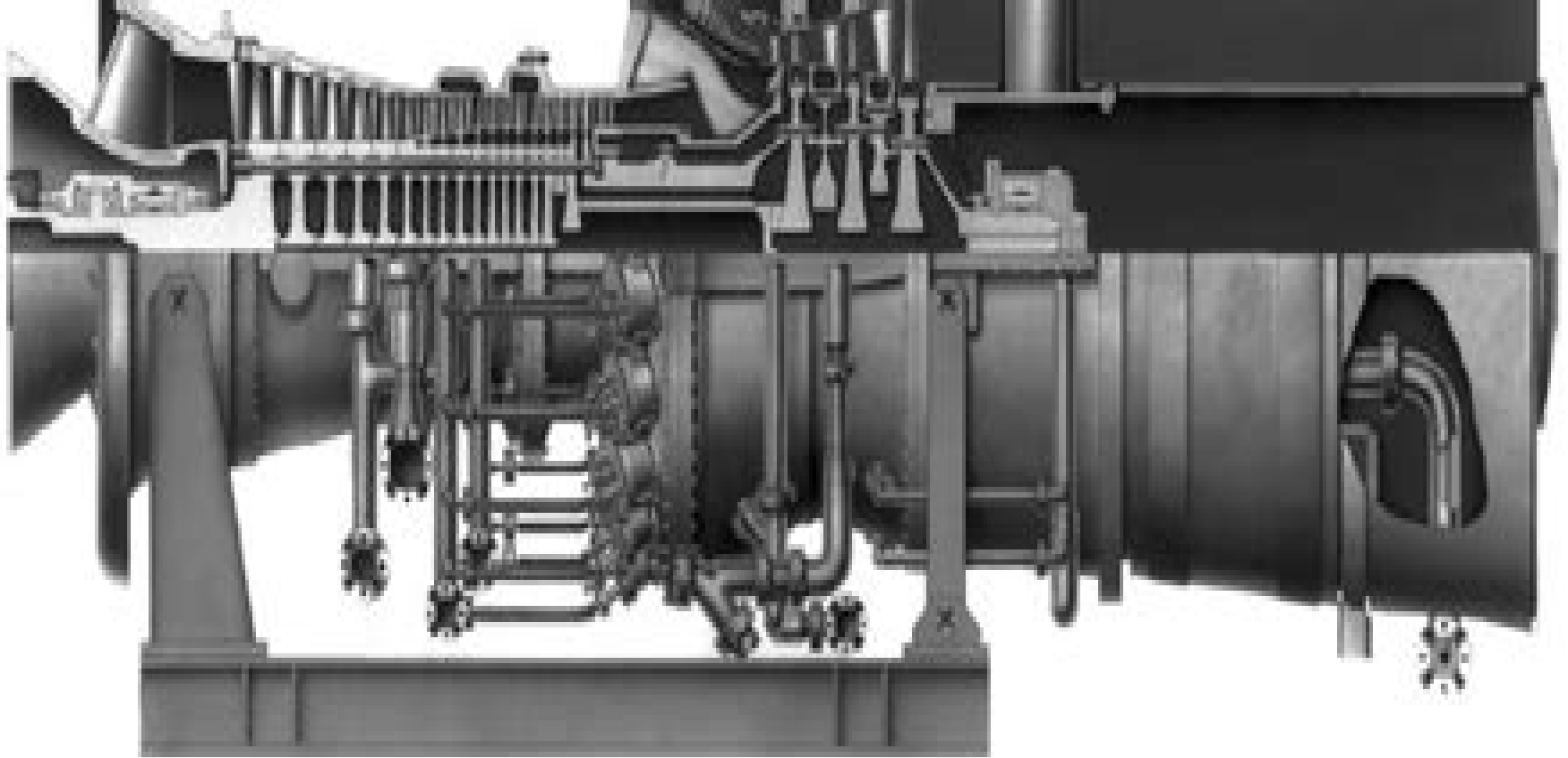
Figure 1-8. A frame type gas turbine with can-annular combustors. (Courtesy GE Power Systems.)
