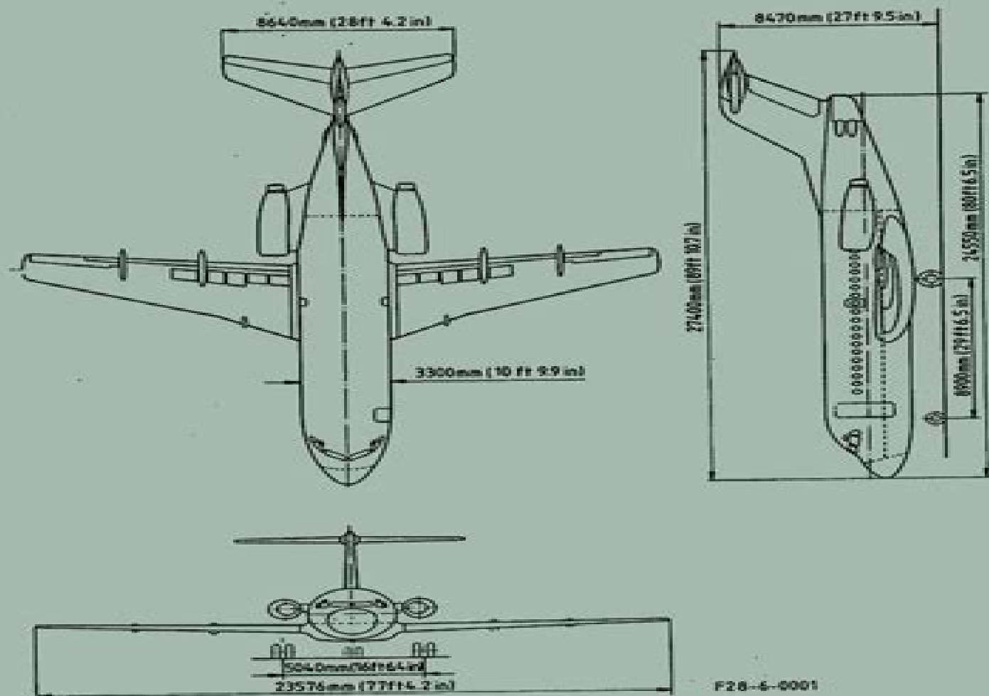
FIG. 2 AIRCRAFT MAIN DIMENSIONS (Sheet 1 of 4) (Mk 1000 and Mk 1000C)
