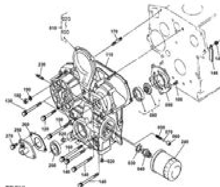
Gear Case
