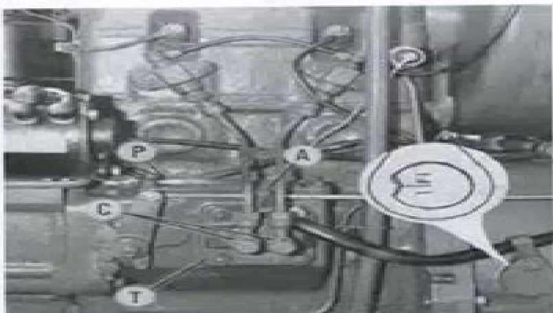
Fig. 50— Installed view of injection pump on Model L210. Inset shows flywheel timing mark for number 1 piston firing position.
