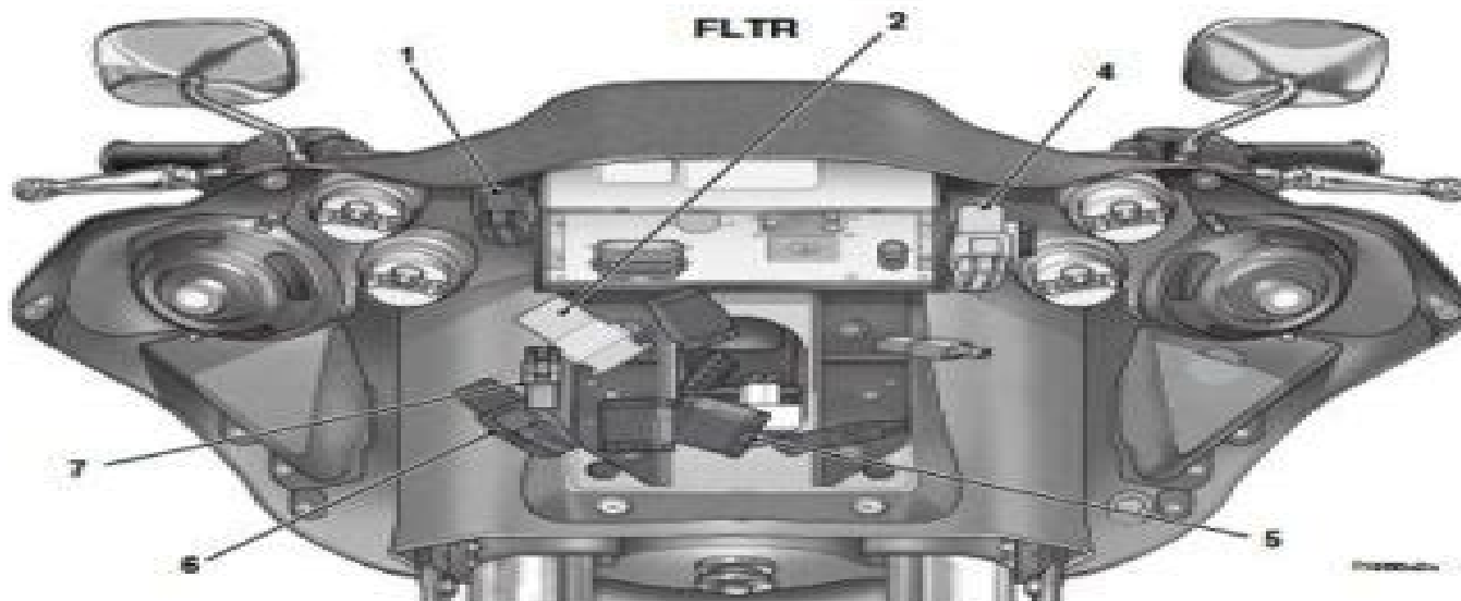
Figure 7-9. Outer Fairing Removed
