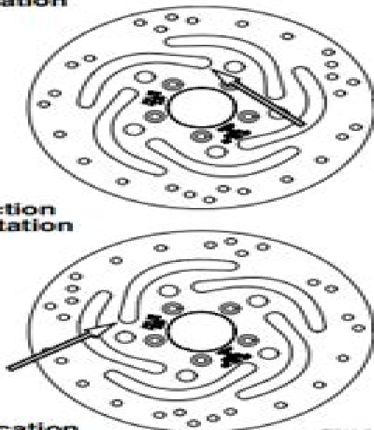
Figure 2-9. Note Bulb Shaped End of Slot (Left Side Brake Disc Shown)
