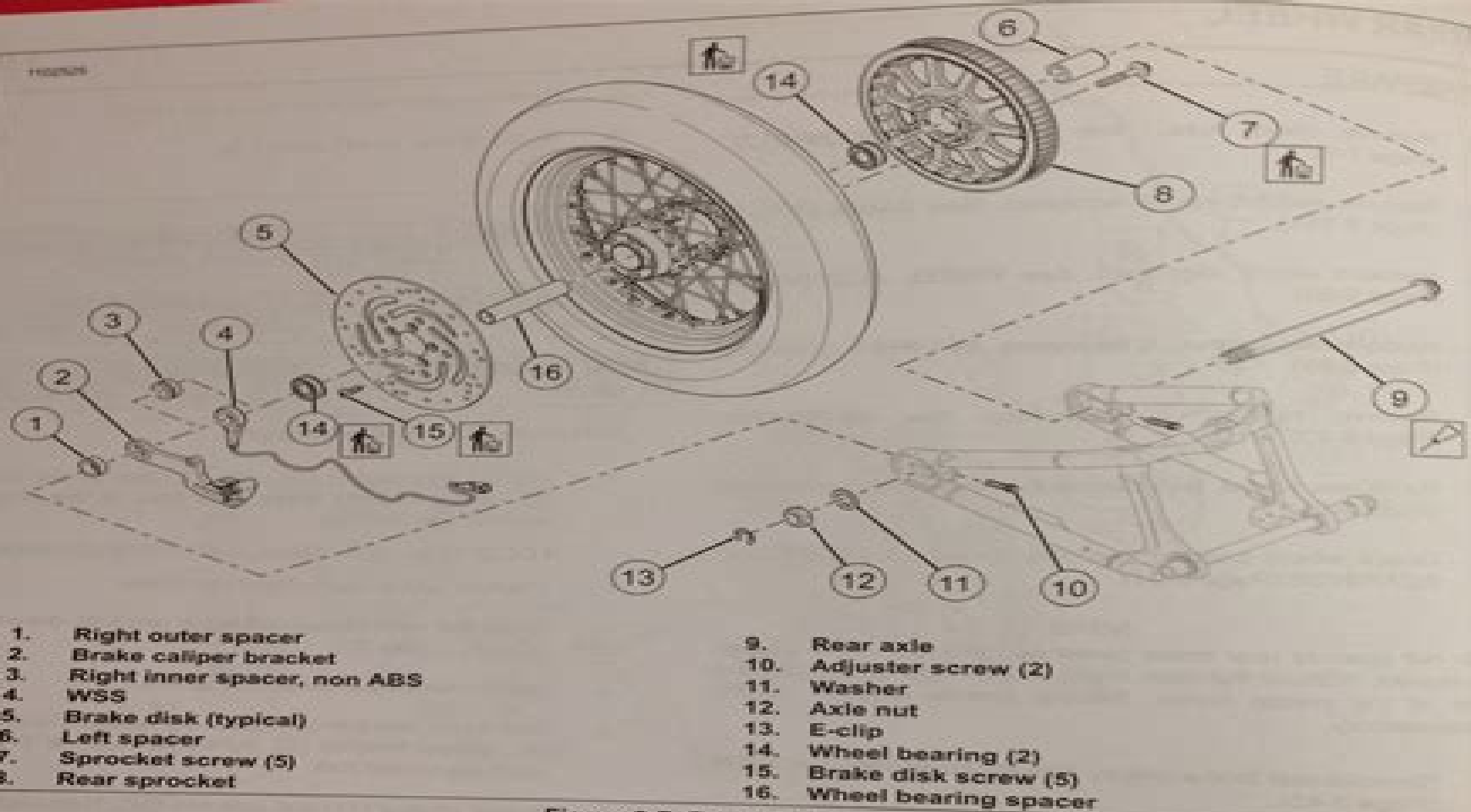
Figure 3-7. Rear Wheel
