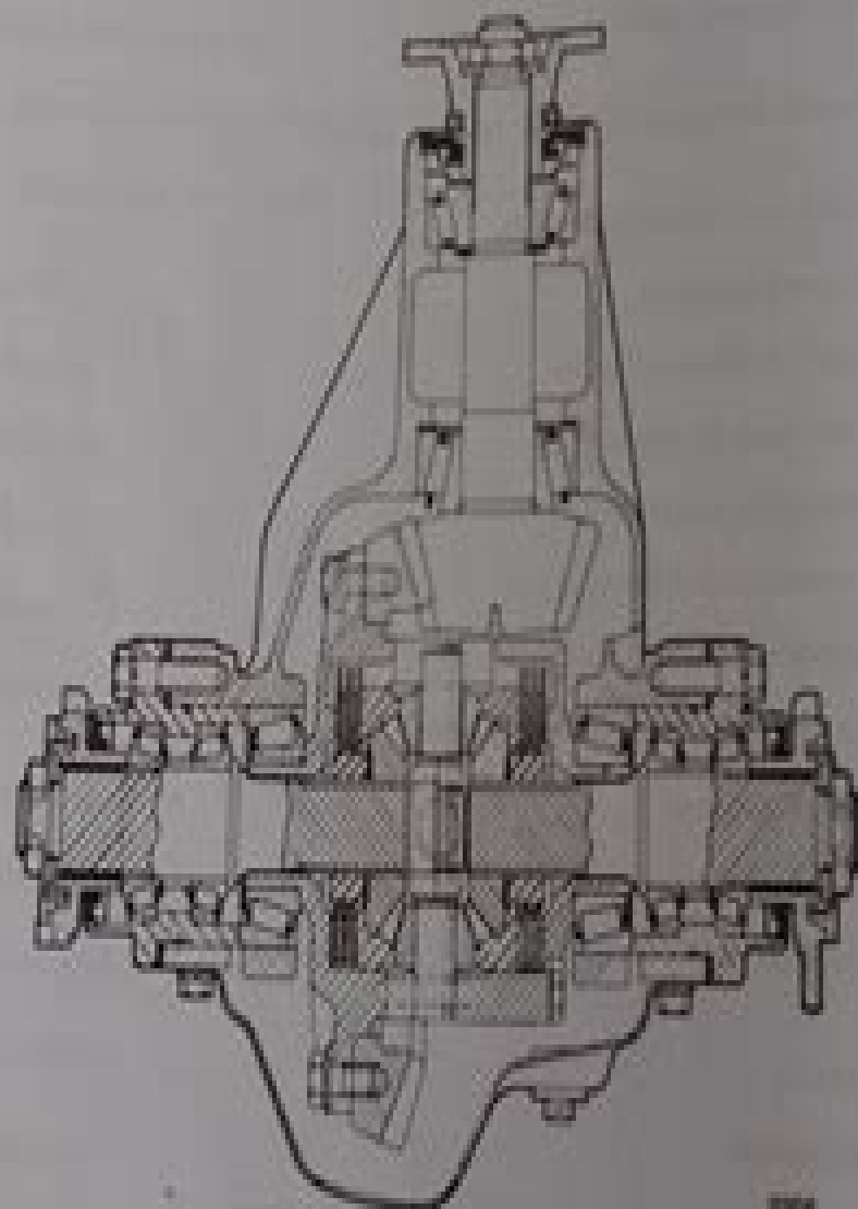
Fig. 1. Sectioned view of the axle unit
