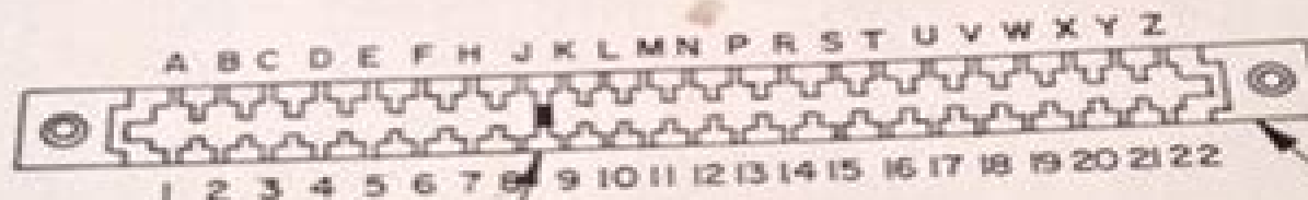
KMA 24H FRONT VIEW
