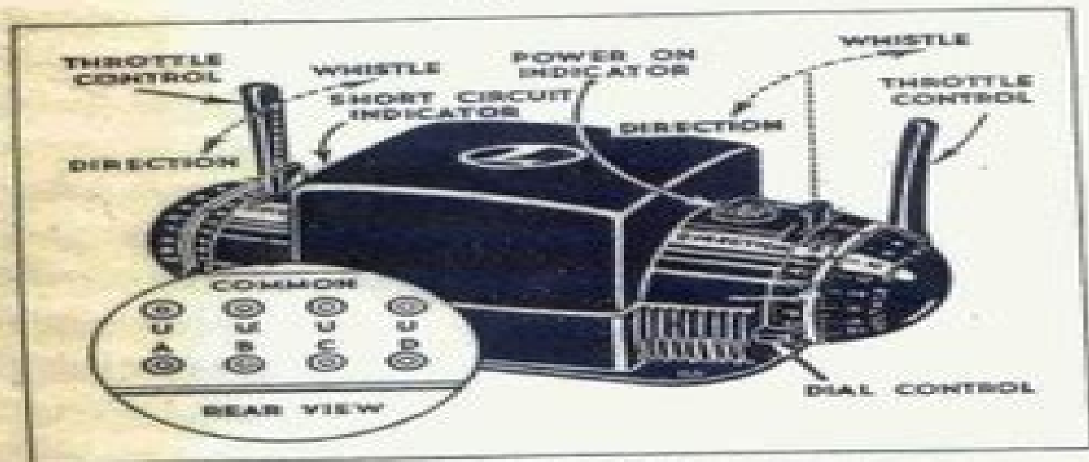
Figure 1—Type ZW "Multi-Control" Transformer.
