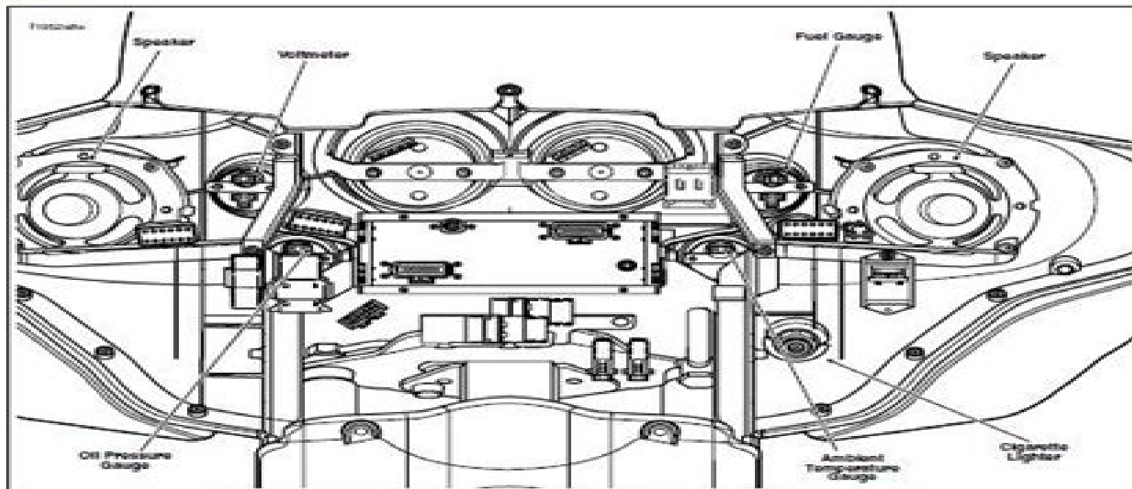
Figure 8-145. Inner Fairing - Interconnect Harness Connectors (FLHTC/U)
